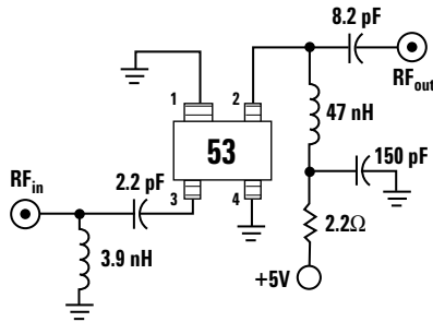
Figure 30. Schematic for 1900 MHz LNA design.
