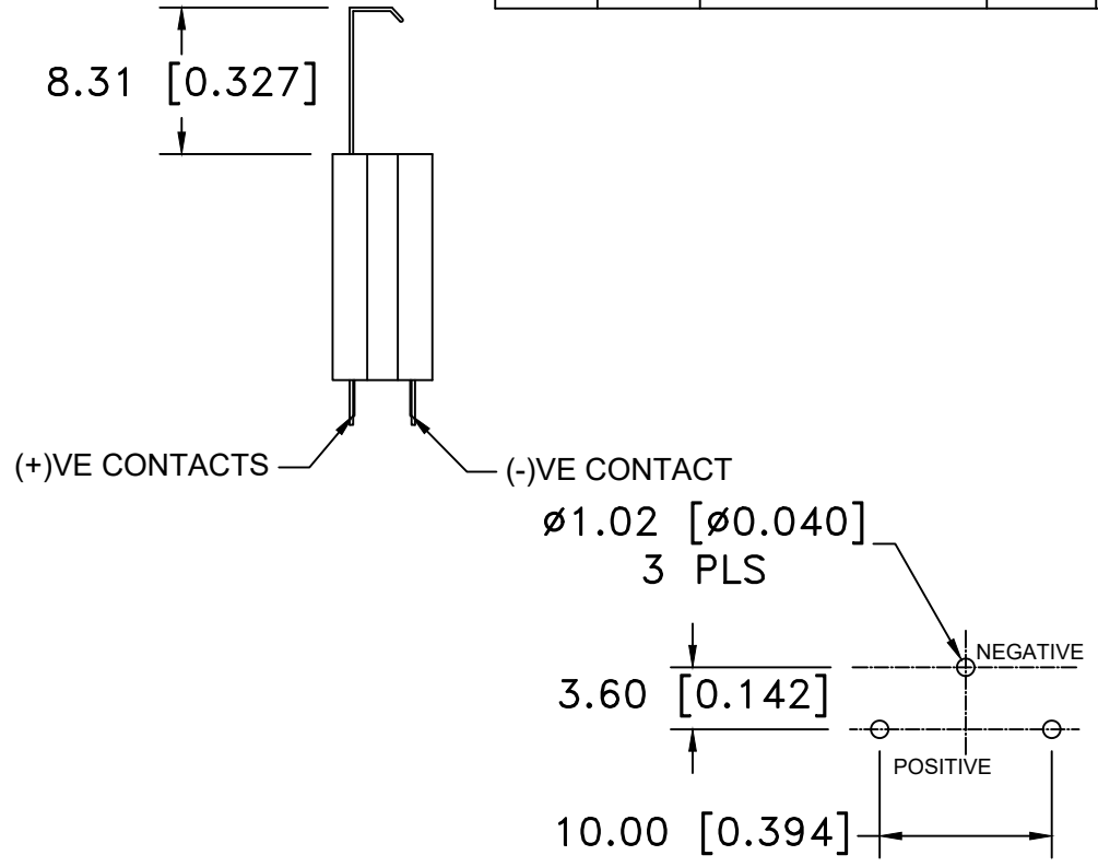
PCB LAYOUT
