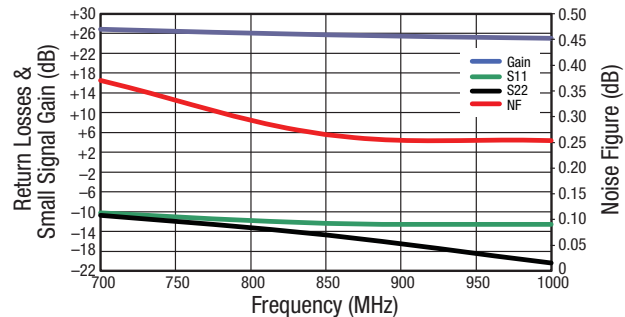
Figure 16. Evaluation Board NF, Gain, and Return Losses for 700 to 1000 MHz Tuning
